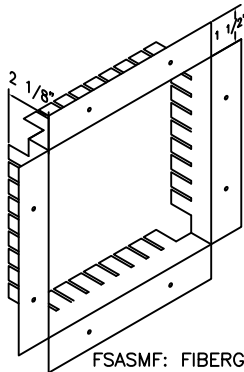
FSASMF: FIBERGLASS DUCT MOUNT FRAME
